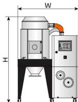
SDD-300U/200H~1200U/700H
