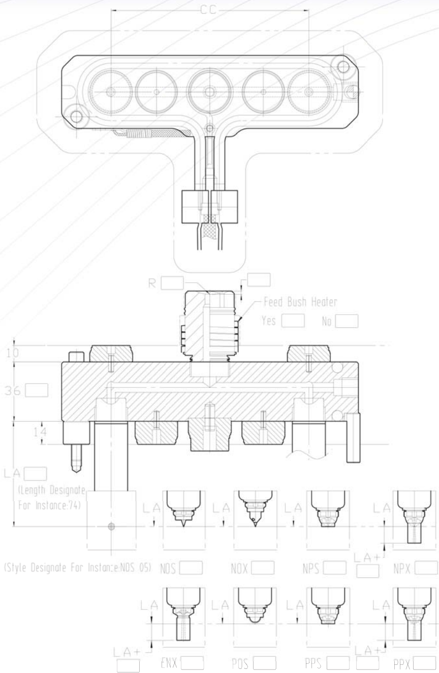
Standard Manifold Styles
