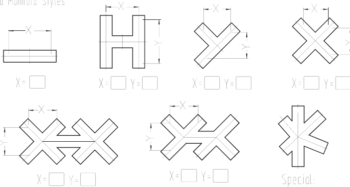
Standard Manifold Styles
